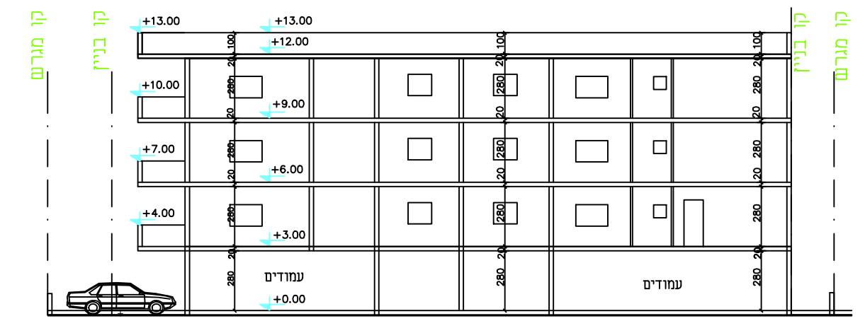
חתך א א 1:250
