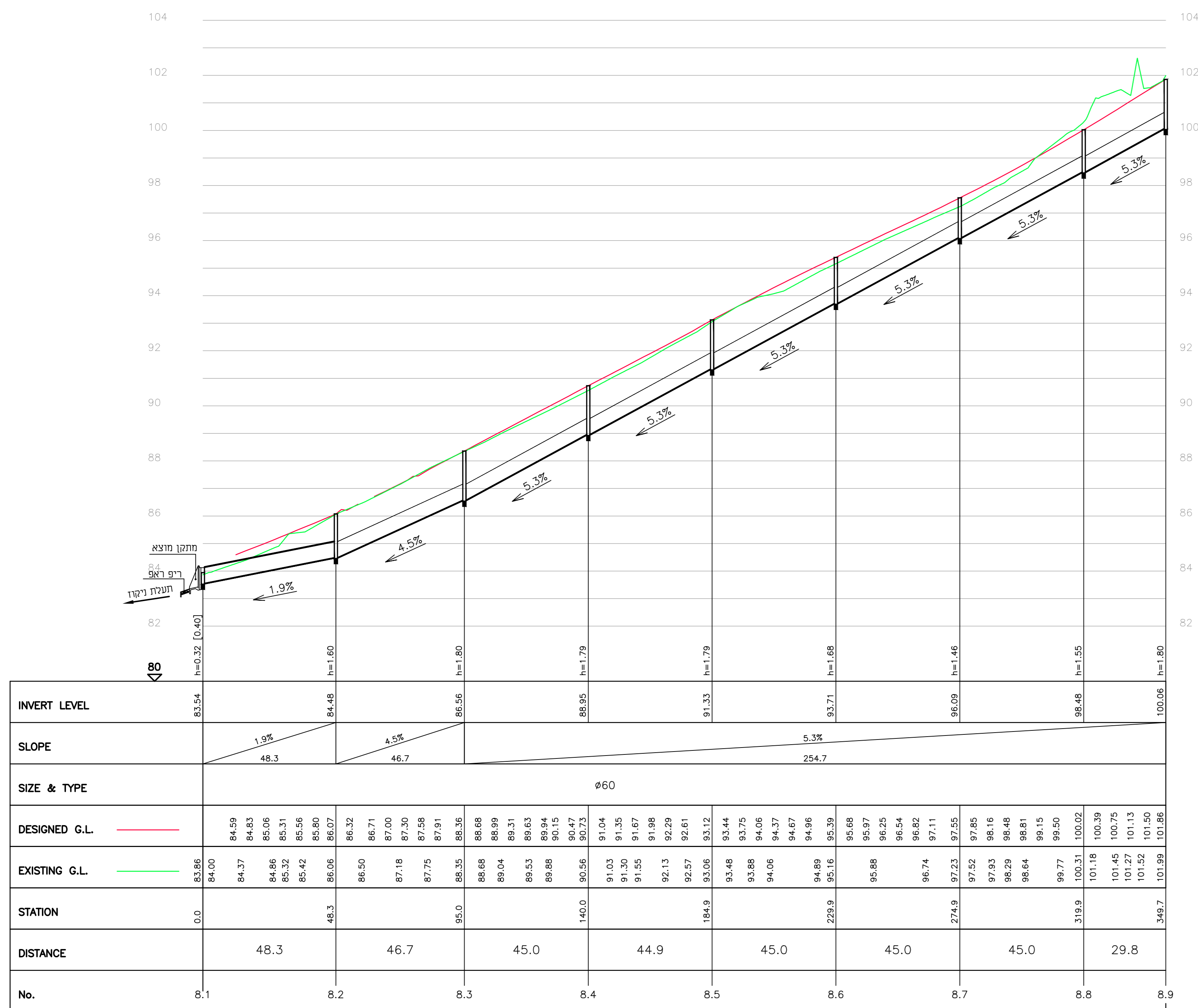
Pipeline Dr1 - 1:100/1:1000 File path: F:\Projects\7021\Civil\Dr1.dxf
